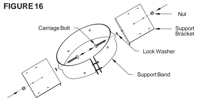
FIGURE 16 Roof Support Assembly
