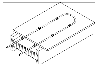
suspended installation using LockDowns™ spaced 32" max (RadiantPEX+) or 60" max (RadiantPEX-AL)
