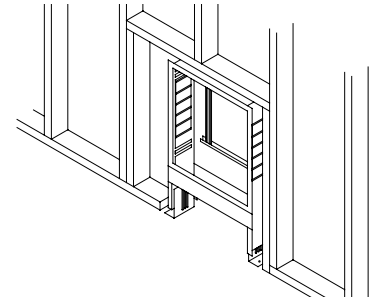
Manifold boxes are designed to be recessed into a standard frame wall. Some framing modifications may be required to accommodate the width of the manifold box.
