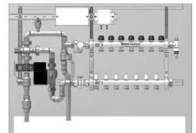
Z-Panel with circulator and mix valve.
