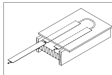
extruded plates place 8" oc with 2-4" gap, used with either RadiantPEX or RadiantPEX-AL
