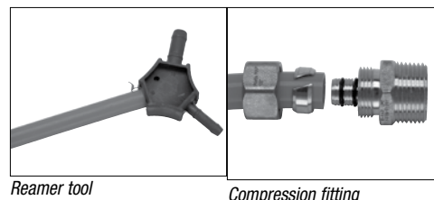
Compression fitting
