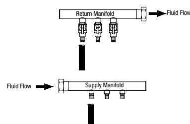
manifold reverse-return piping configuration
