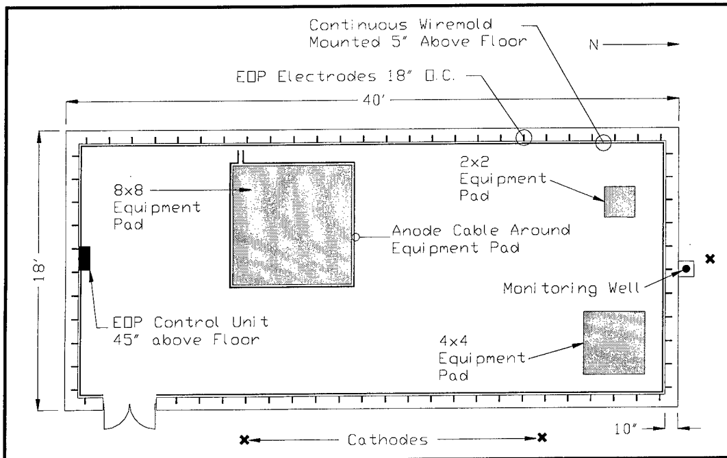
Figure 9. Layout of EOP installation at Fort Jackson.
